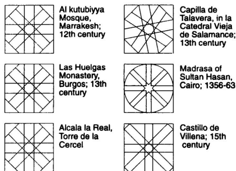
8-pointed star ribbed domes, type (8/3)3 with extended ribs
